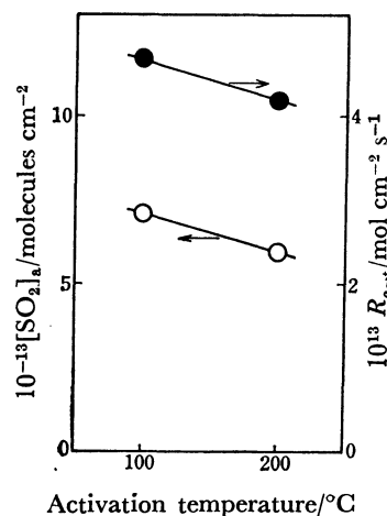
Fig. 6. The amount of weakly adsorbed SO 2 and the rate of isomerization of cis -2-butene on Mg(OH) 2 as a function of pretreatment temperatures: (●); the rate of cis -trans isomerization, (○); the amount of weakly adsorbed SO 2 . \theta_s = 0.57.
