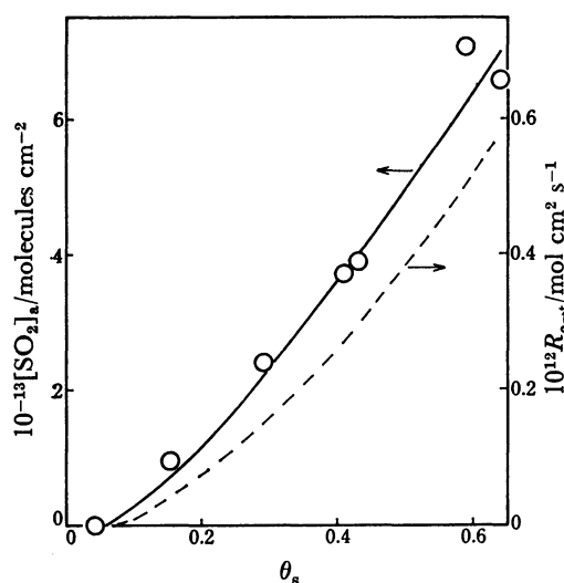
Fig. 4. The amount of weakly adsorbed SO 2 and the rate of cis -trans isomerization of cis -2-butene on Mg(OH) 2 , as a function of \theta_s : The sample was activated at 100 °C. —; The amount of weakly adsorbed SO 2 , ---; the rate of cis -trans isomerization.
