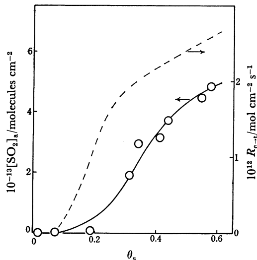
Fig. 5. The amount of weakly adsorbed SO 2 and the rate of isomerization of cis -2-butene over MgO as a function of \theta_s : The sample was activated at 400 °C. —; The amount of weakly adsorbed SO 2 , ---; the rate of cis -trans isomerization.
